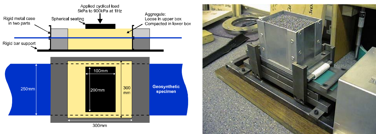
Figure 7: ENV ISO 10722 - Procedure for simulating damage during installation
