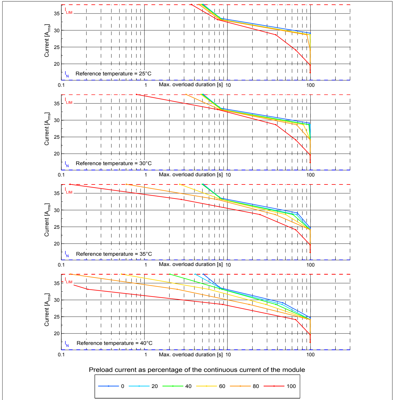
Figure 1: 8BVI0110HWSx.000-1 - Overload characteristics, overload response - WARNING
