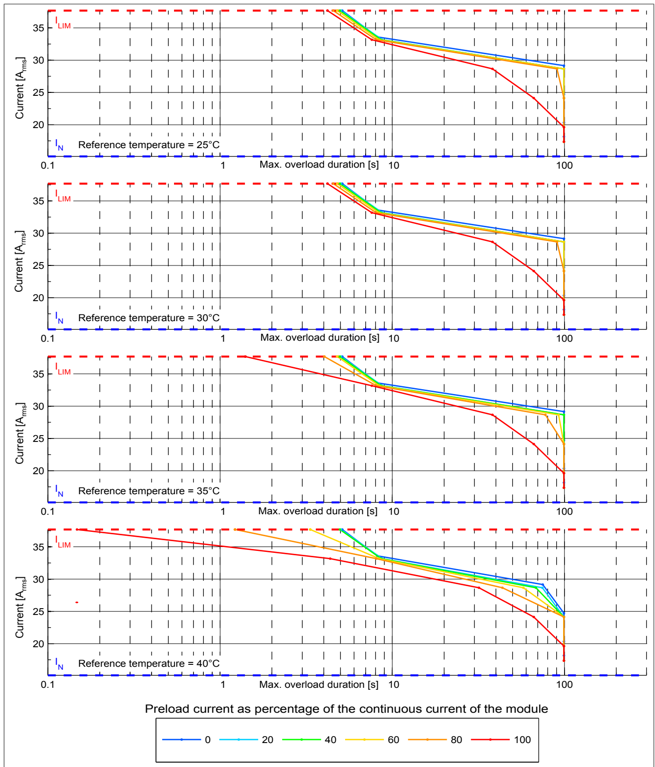
Figure 2: 8BVI0110HWSx.000-1 - Overload characteristics, overload response - ERROR+STOP
