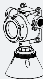
Collecting Cone
