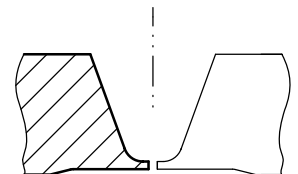
J-Prep Bevel
