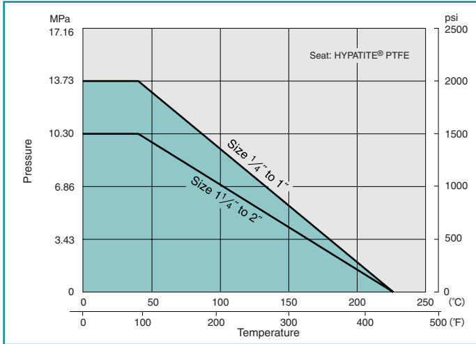
Type 1500/2000: AKSCTHZM/AKSCTHWZM/AKUTHZM/AKUTHWZM
