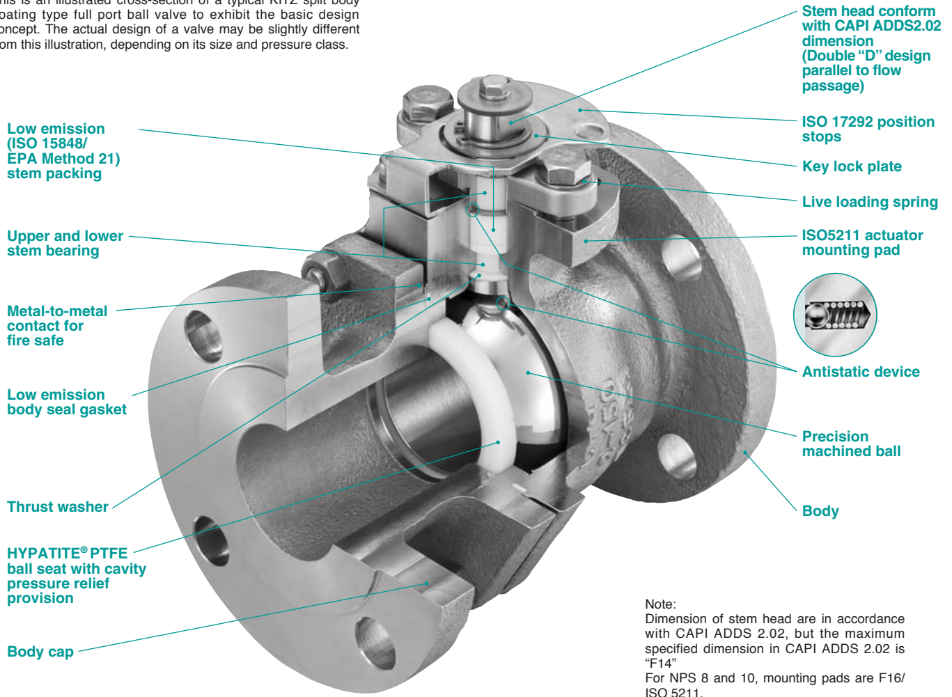
2" KITZ 150UTDZ
