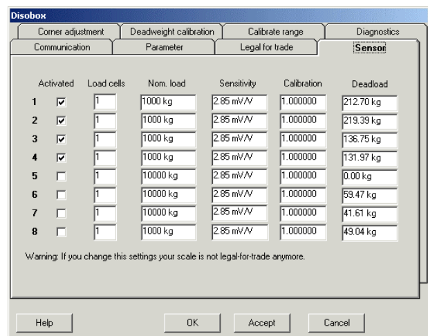
Fig. 4: Configuration of Load Cell on a DISOBOX® Scale
