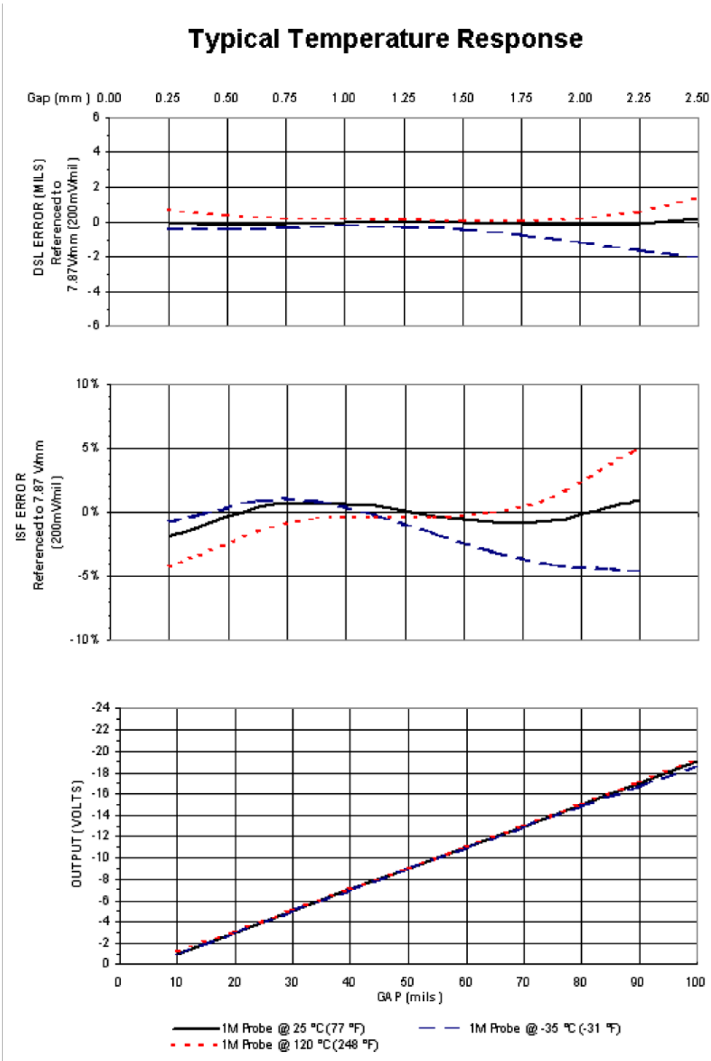
Figure 2: 3300 5 Meter XL Proximitor Sensor at High Temperatures (3300 5mm Probe and XL Extension Cable at 25°C)
