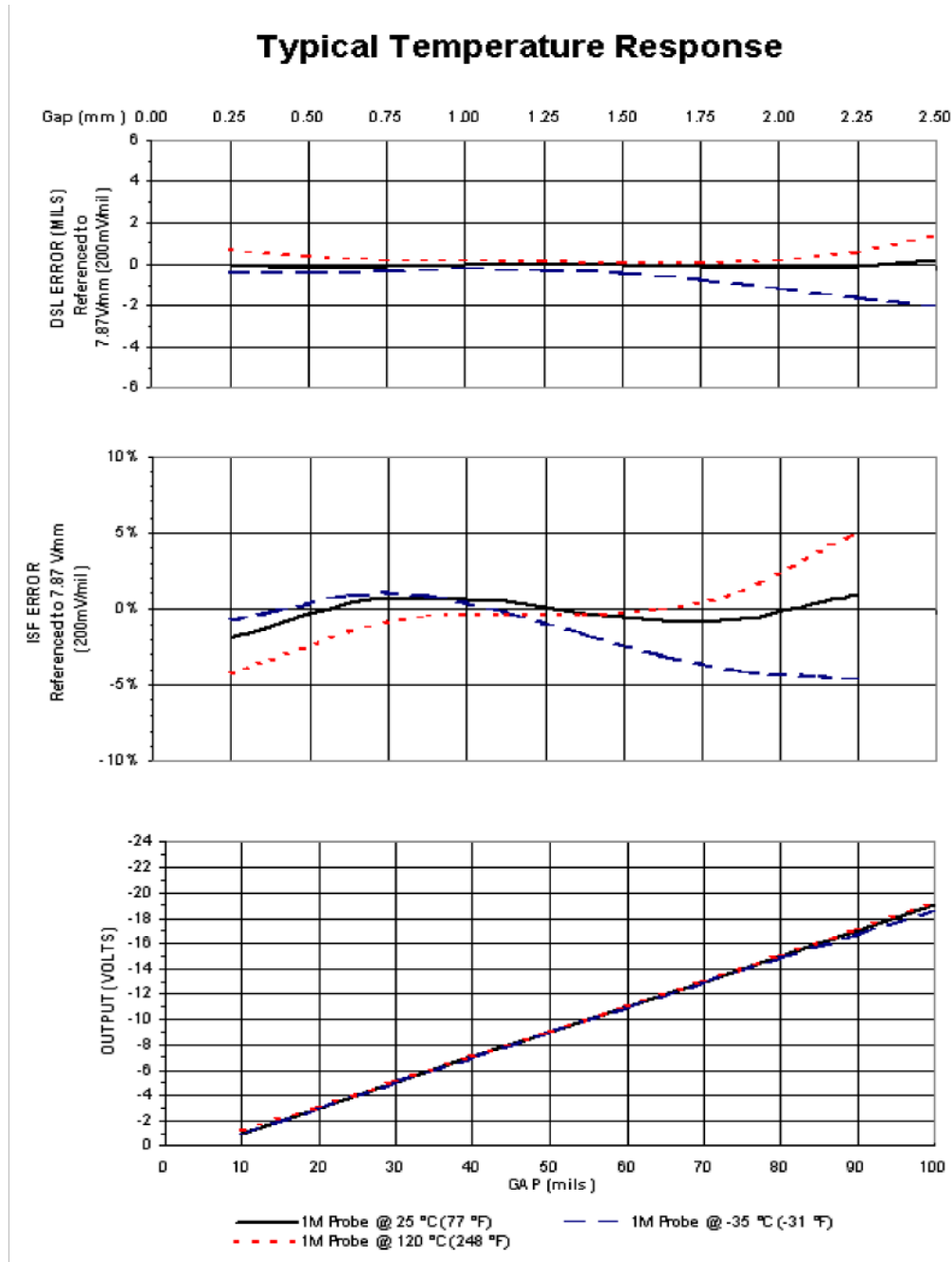
Figure 1: Typical 3300 5mm Probe and 1 Metre of Cable at High and Low Temperatures (XL Proximitor Sensor and XL Extension Cable are at 25°C)
