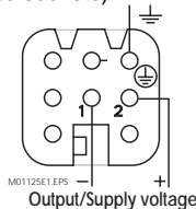
Crimp terminal for 0.75...1,0mm 2 conductor (also solderable) Fig. 10. Connection diagram for socket connector
