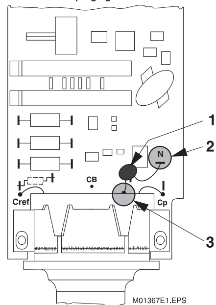
1 Capacitor C22 2/3 unsolder
