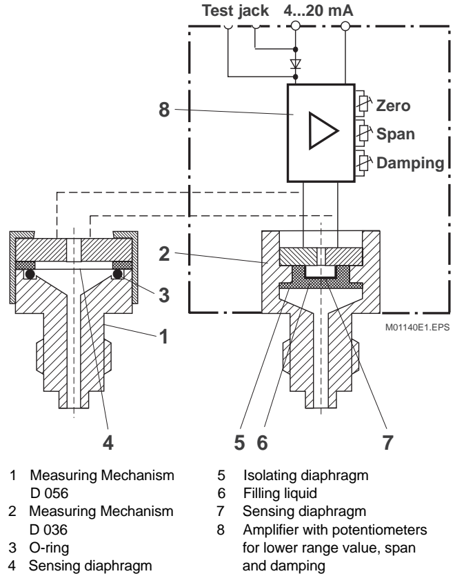
Fig.1. Functional Diagram
