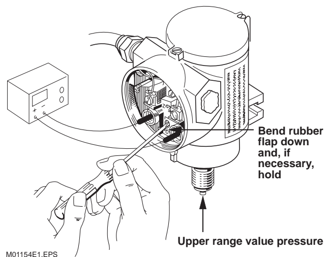
Fig. 17. Correcting the upper range value
