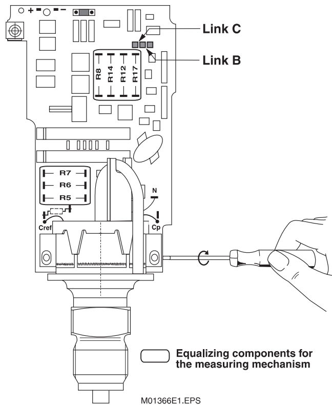
Fig. 34. Component side of the measuring mechanism/electronic unit of the AMD 220
