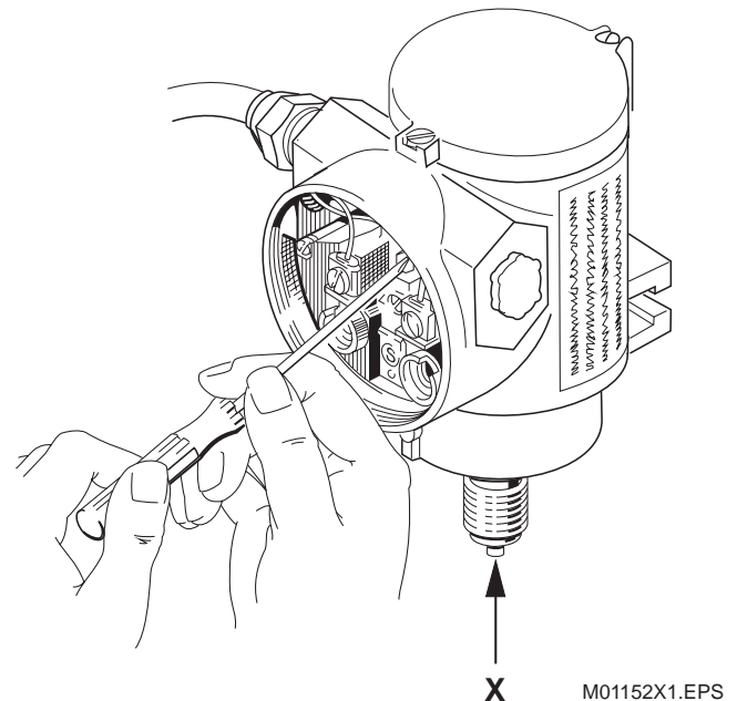
Fig. 14 Adjusting the damping using a screwdriver
