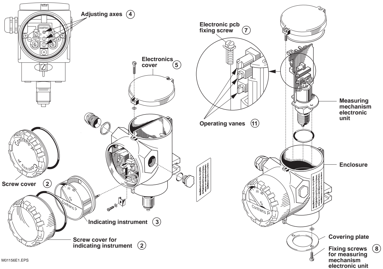
Fig. 18. Exploded view e.g. AMD 200
