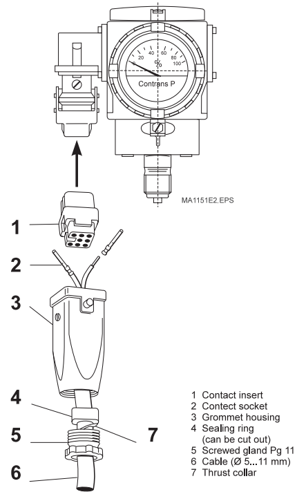
Fig. 11. Installing the socket connector
