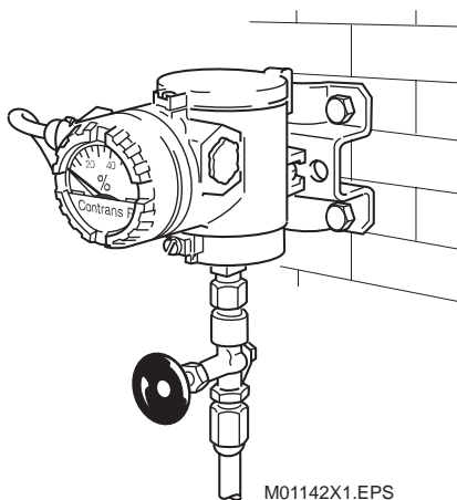
Fig. 3. Wall mounting with mounting bracket
