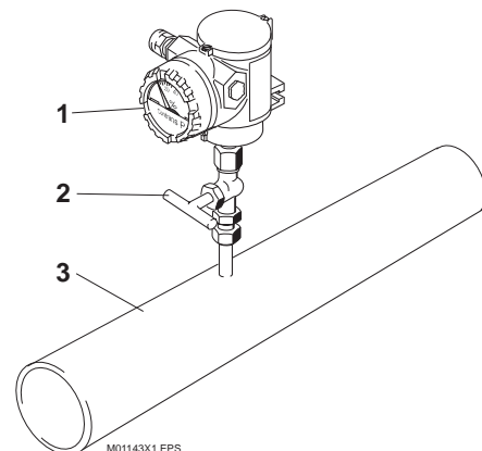
Fig. 4. Direct mounting
