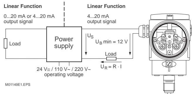
Fig. 13. Connecting to a power supply
