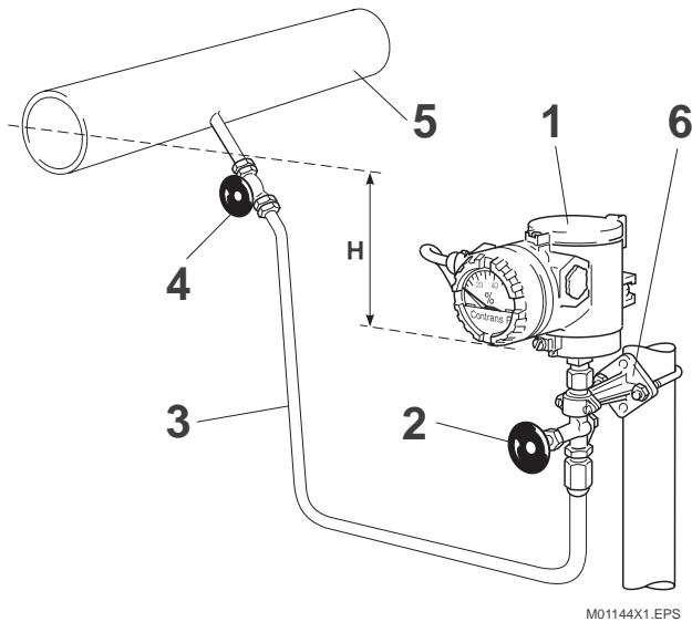
Fig. 7. Example of measuring arrangement for vapour measurement
