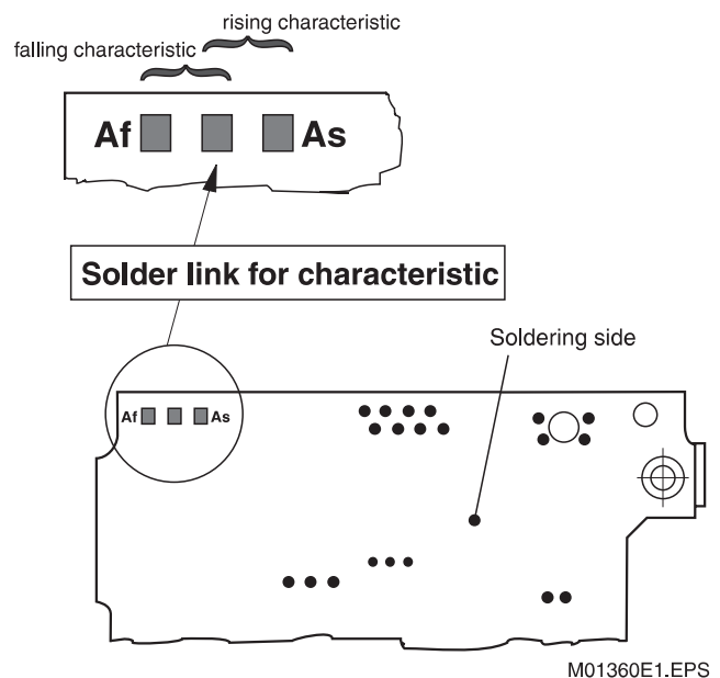
Fig. 22. Position of the "Solder link for characteristic"
