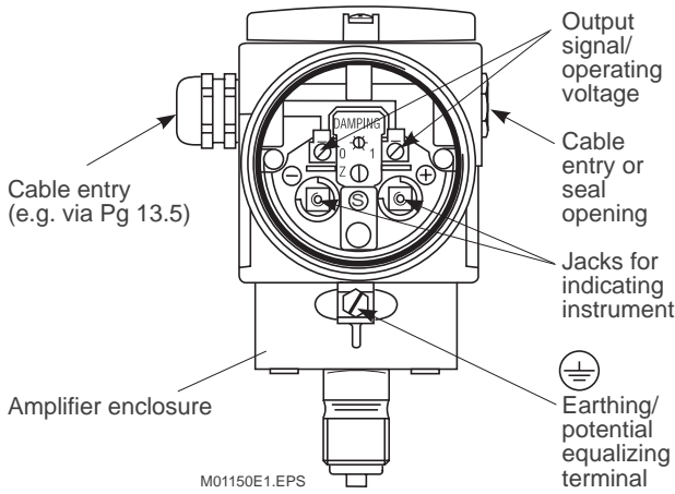
Fig. 9. Cable connection housing
