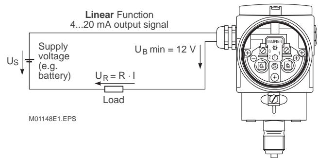
Fig. 12. Connection diagram
