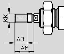
K6 – Shortened male piston rod thread
