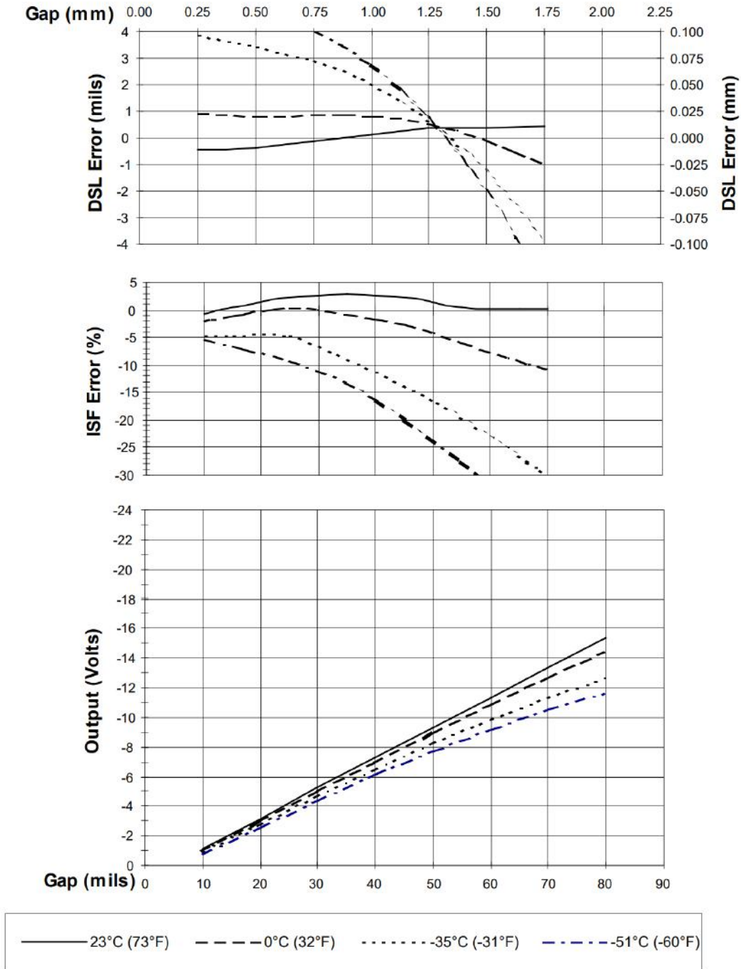
Figure 3: Typical 3300 NSv Probe + 1m Cable @ Low Temperature (Proximitors Sensor + 4m of Extension Cable @ 25 °C)
