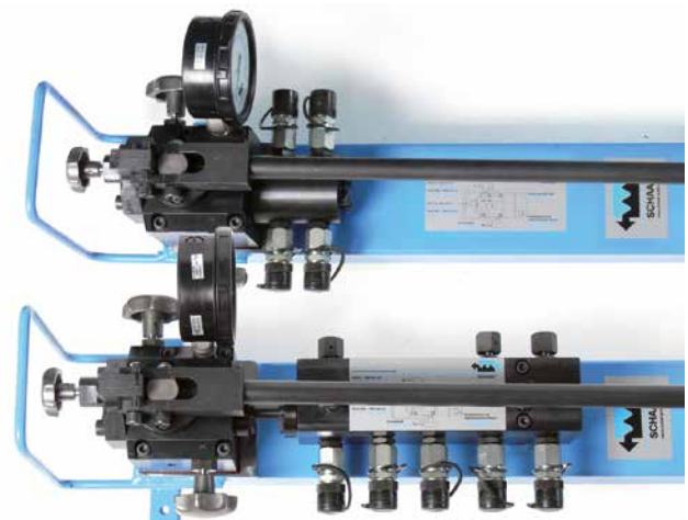
Example (top): HP 1600-2S with 4 outlets Example (bottom): HP 1600-2S with 5 outlets, 3 of these with separately shutoff valve
